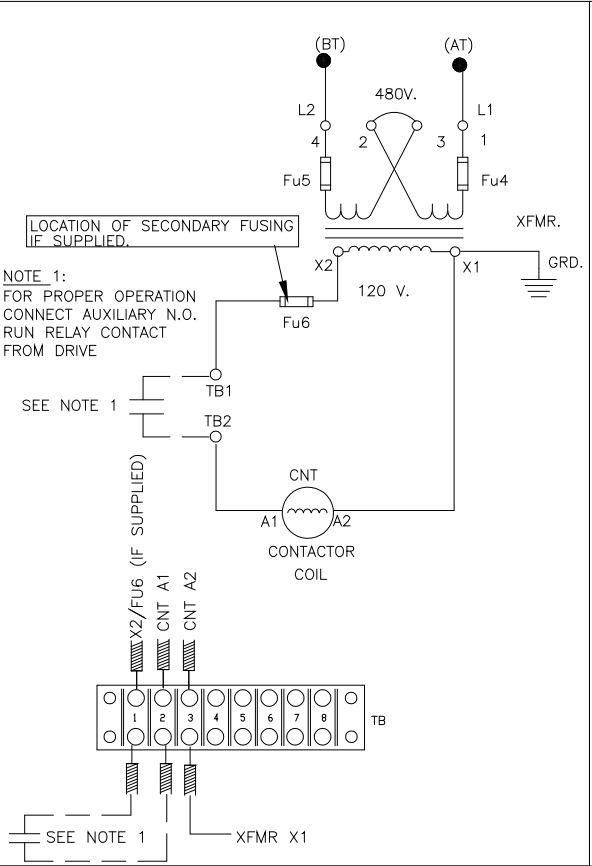
CONTROL CONNECTIONS WITHOUT FAN(S)
