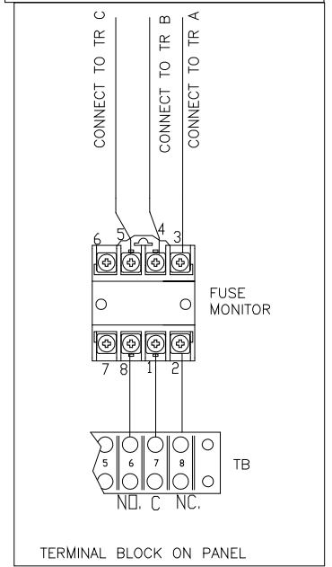
SCHEMATIC FOR FUSE MONITOR, OPTION
