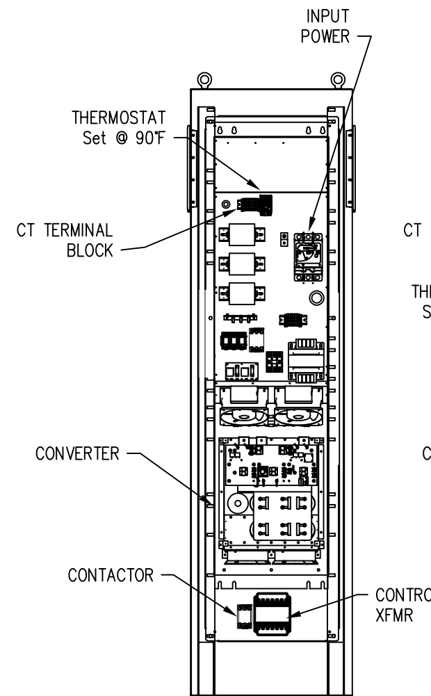
INTERIOR VIEW 150A ASSEMBLY
