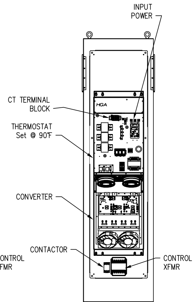
INTERIOR VIEW 50/100A ASSEMBLY
