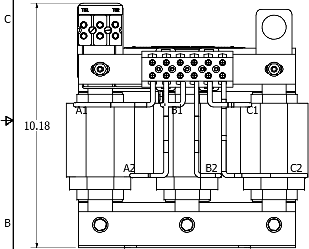
Markings On Coil And Terminal Block For Reference Only.
