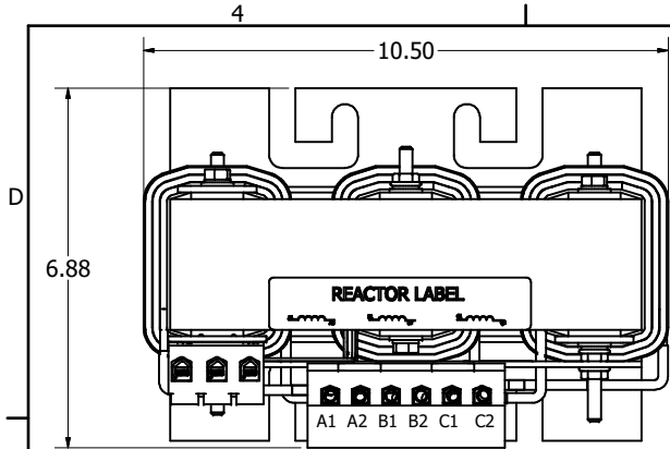
Markings On Coil And Terminal Block For Reference Only.
