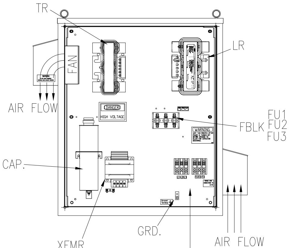
FRONT VIEW WITHOUT DOOR
