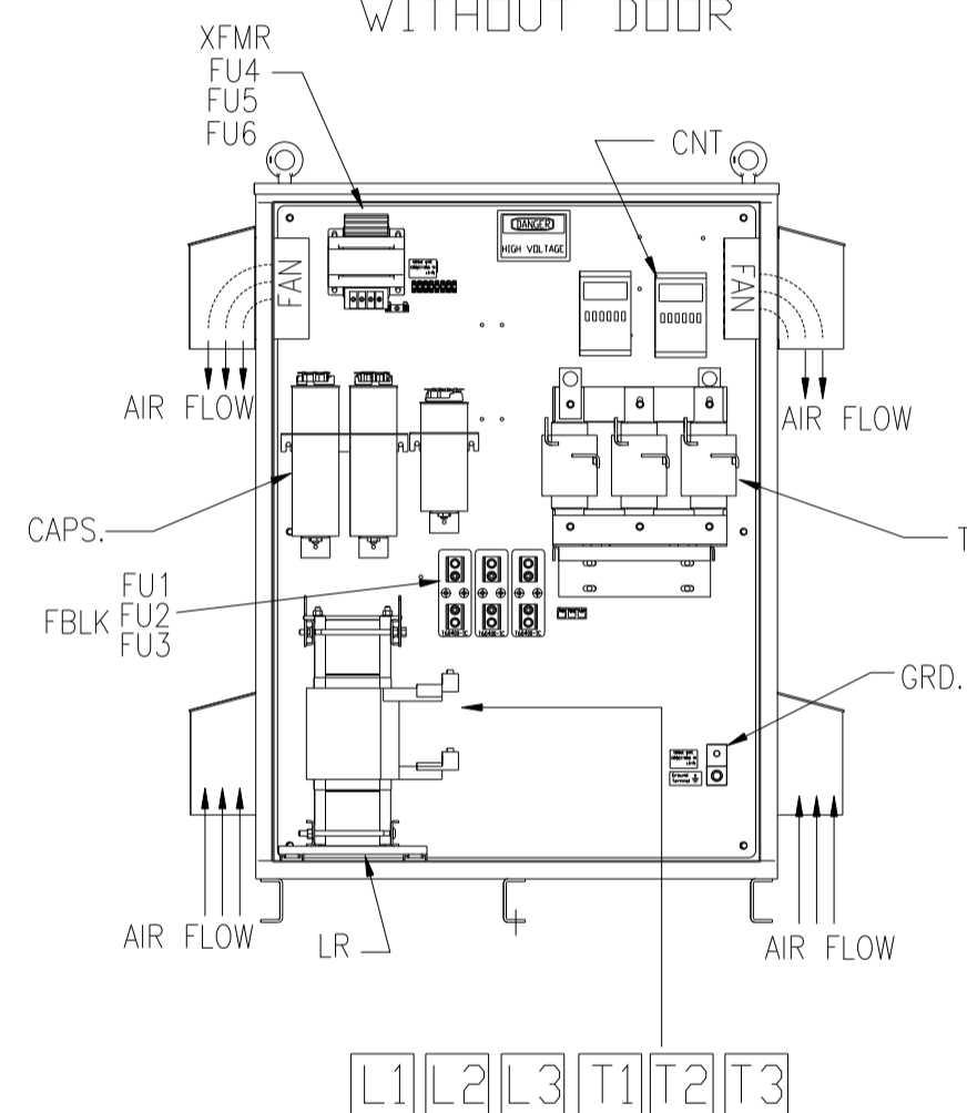
SUGGESTED CUSTOMER WIRE ENTRY AND EXIT LOCATION
