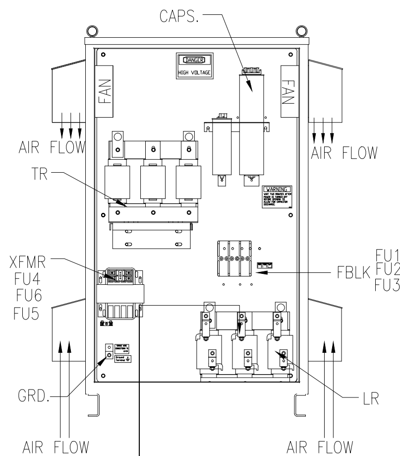
FRONT VIEW WITHOUT DOOR
