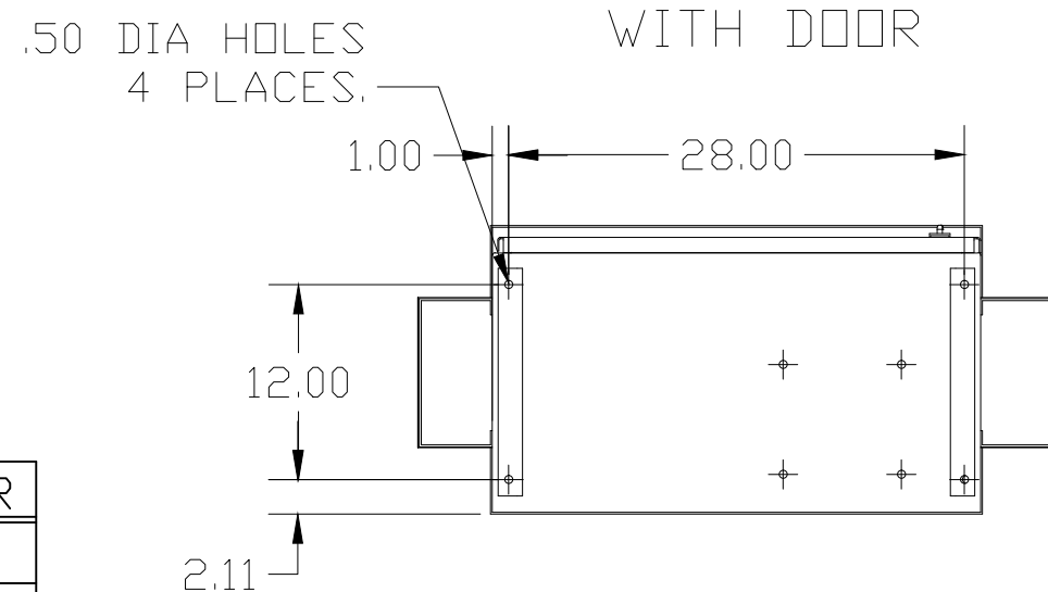
FRONT VIEW WITH DOOR
