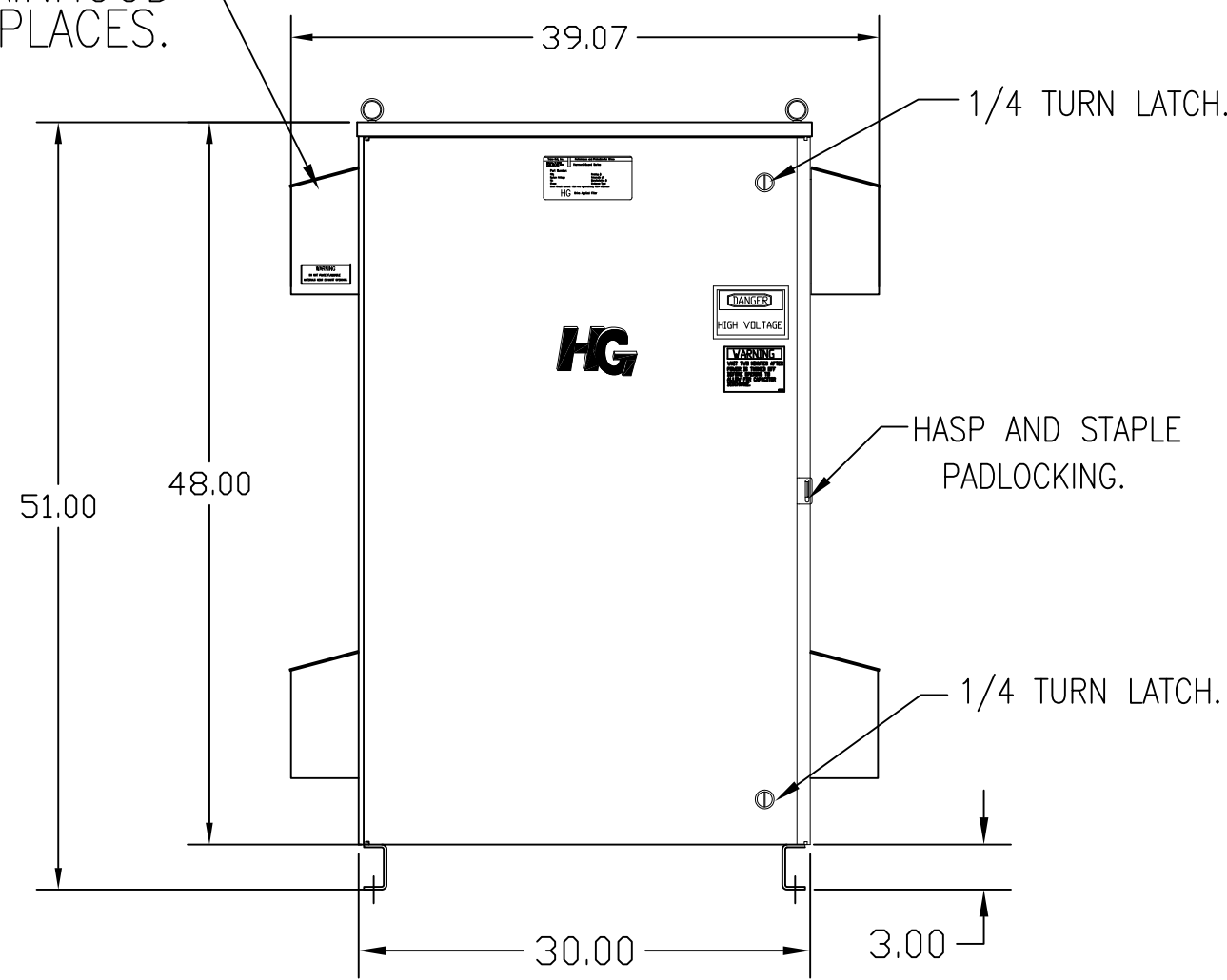
FRONT VIEW WITH DOOR
