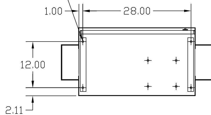
FRONT VIEW WITH DOOR
