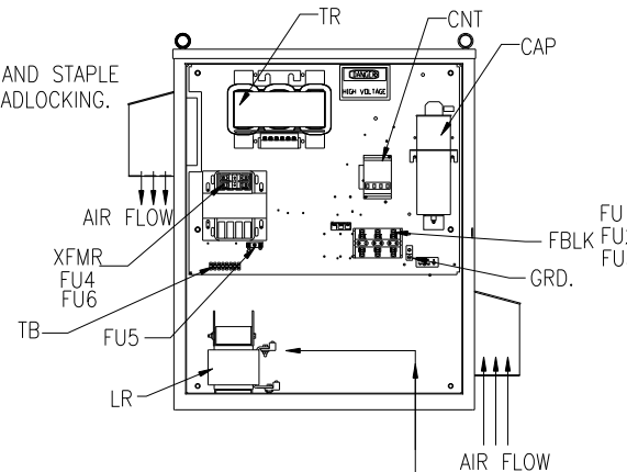
FRONT VIEW WITHOUT DOOR
