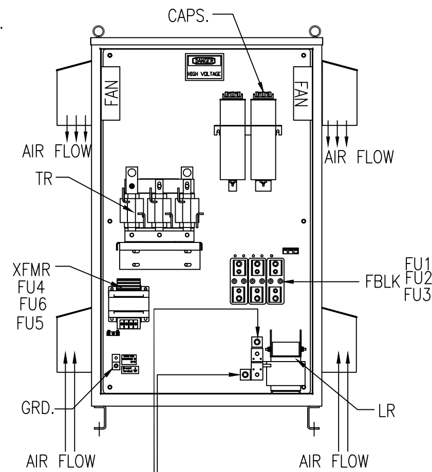
FRONT VIEW WITHOUT DOOR
