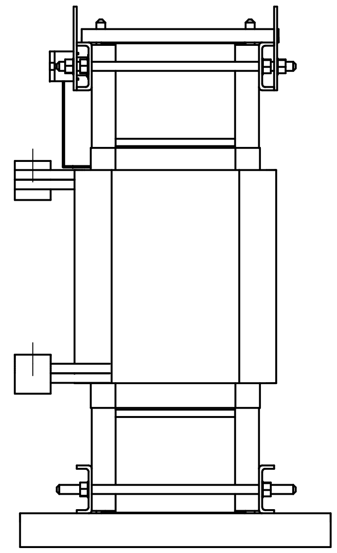
Side View
