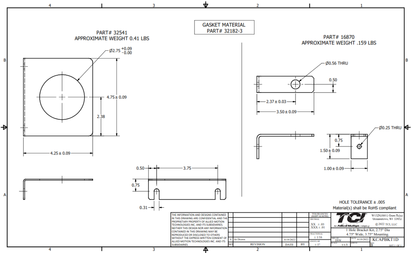
Figure 2: New Capacitor Mounting Bracket KCAPBKT1D
