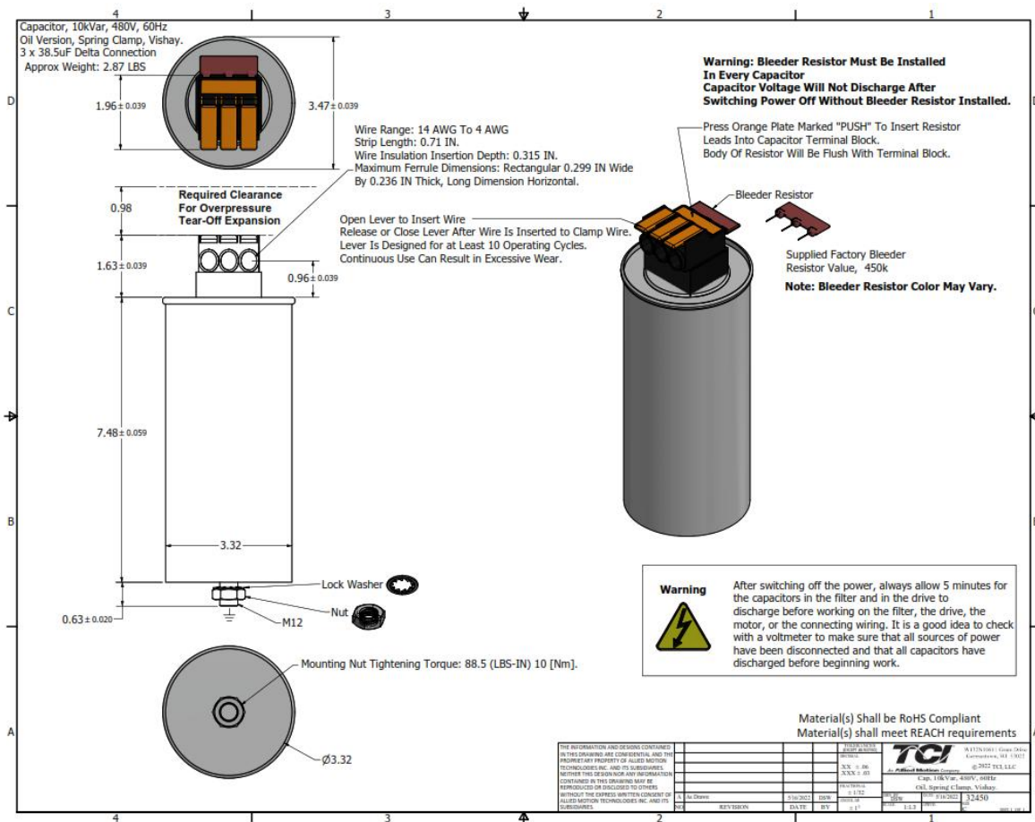
Figure 4: New 10 kVAR Spring Clamp
