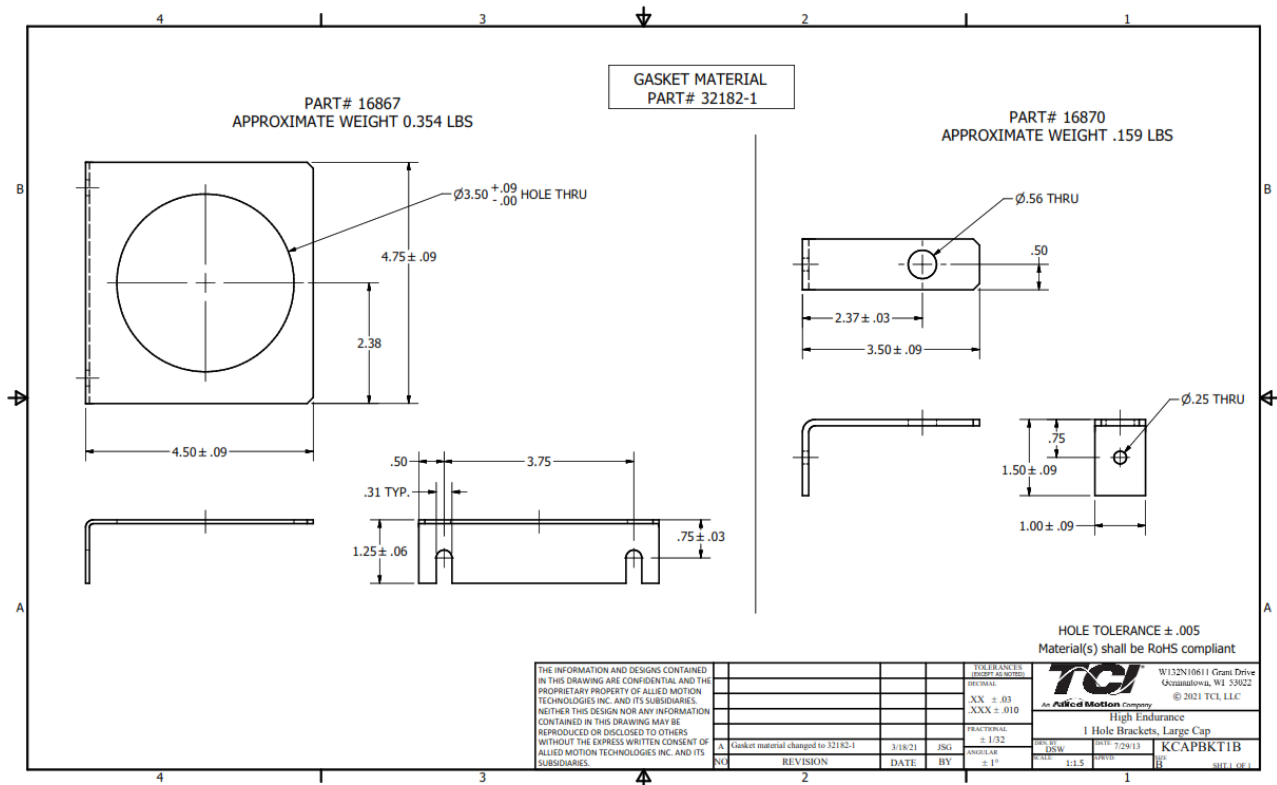
Figure 1: Old Capacitor Mounting Bracket KCAPBKT1B
