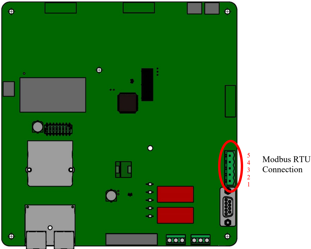
Figure 5 – PQconnect Modbus RTU Connection
