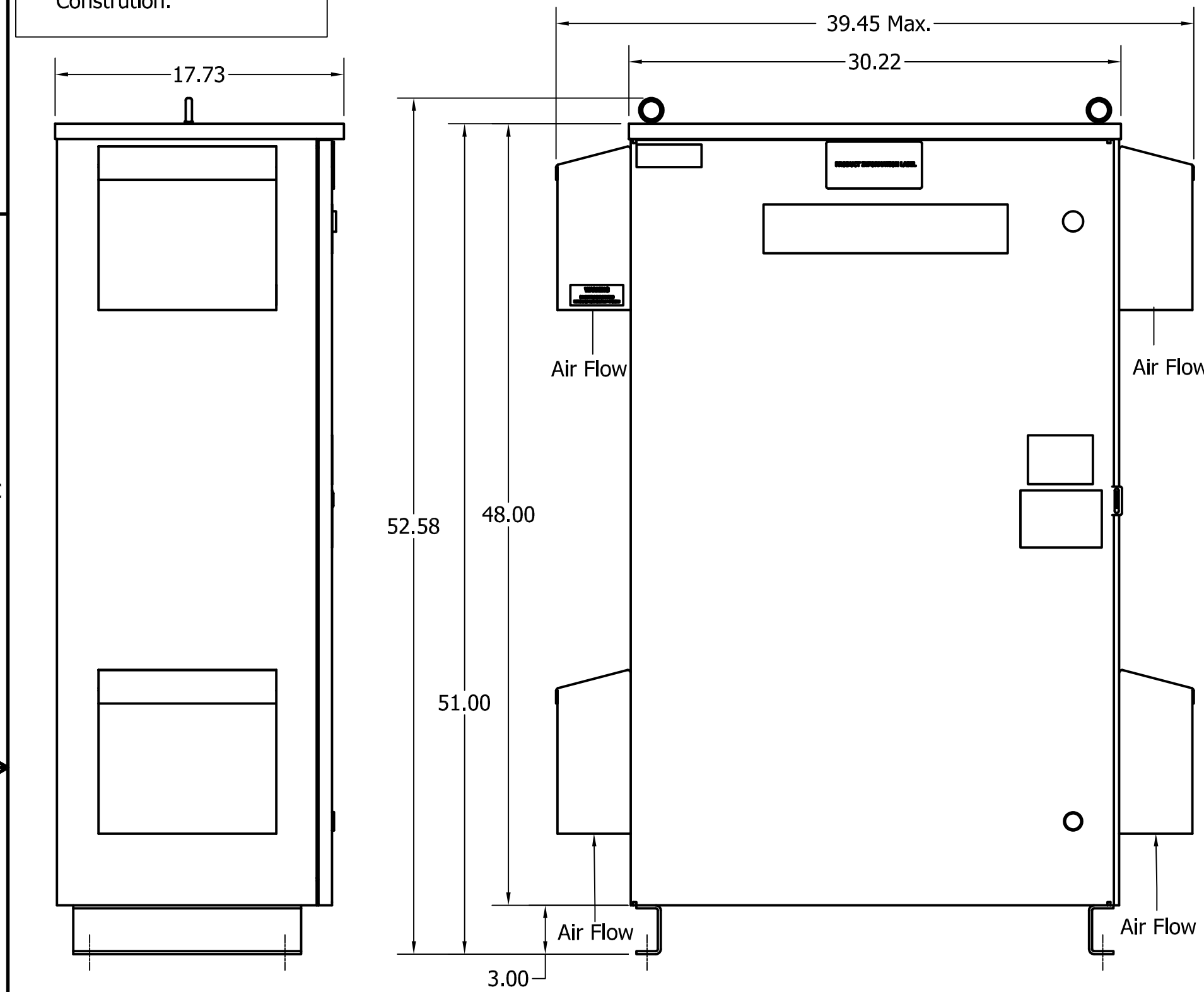
Alternate Rain Hood Construction.
