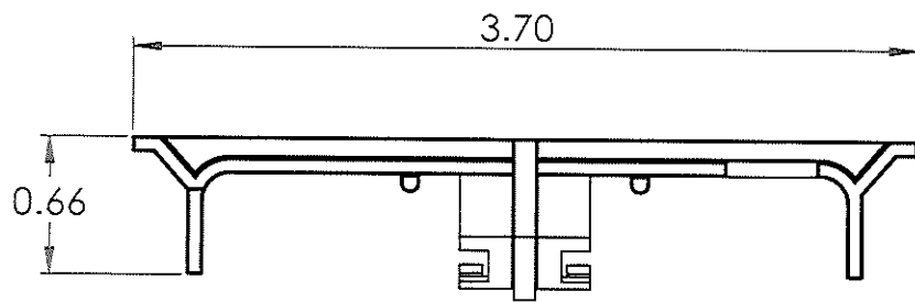
FUSE HOLDER
