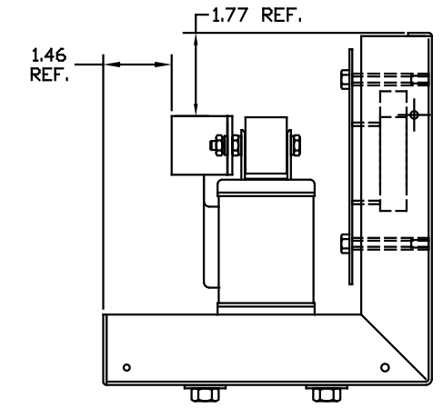
BASE, REACTOR AND BOARD
