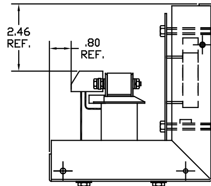
BASE, REACTOR AND BOARD
