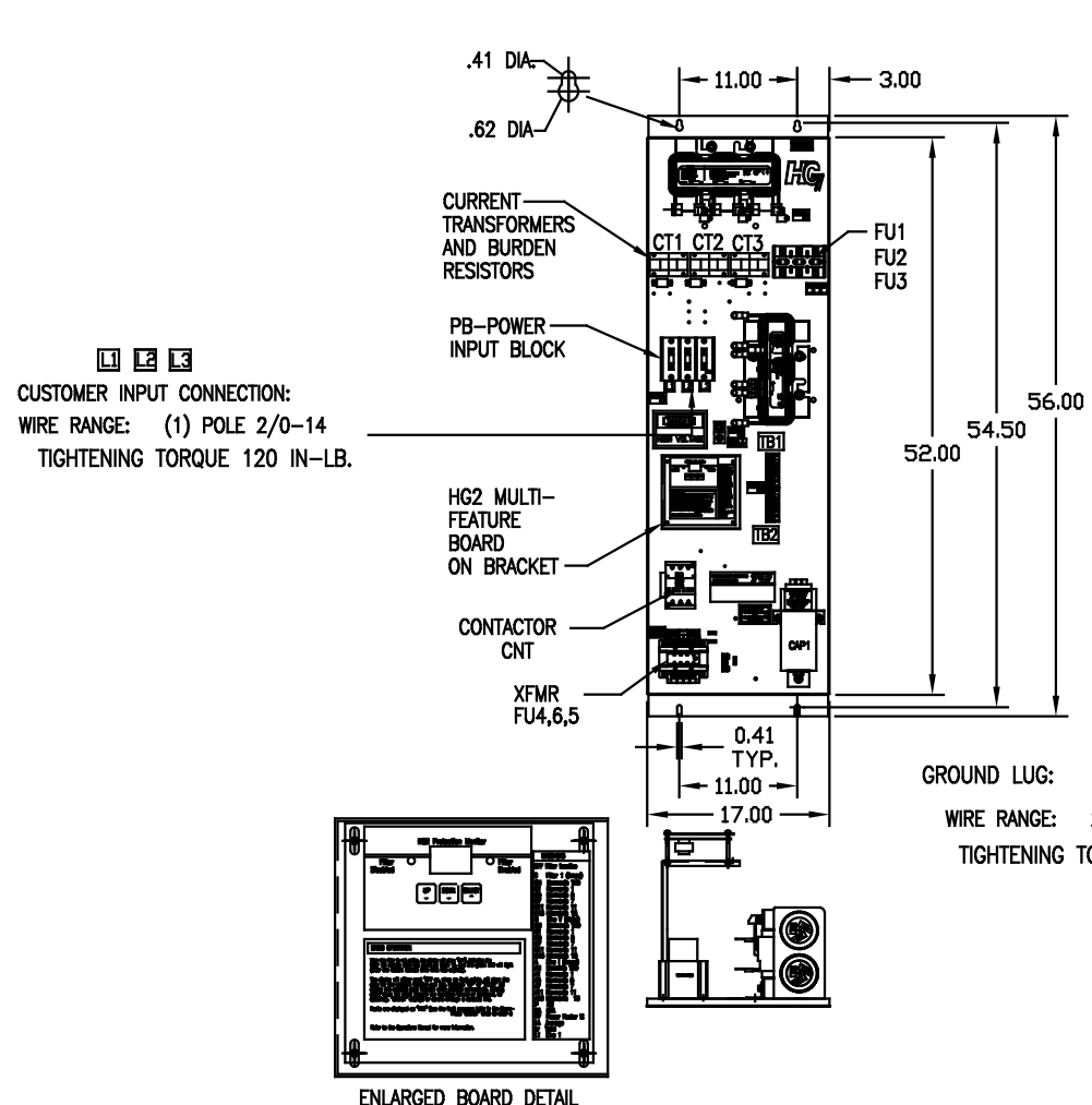
ENLARGED BOARD DETAIL
