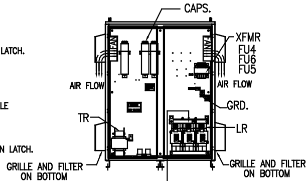
SUGGESTED CUSTOMER WIRE ENTRY AND EXIT LOCATION
