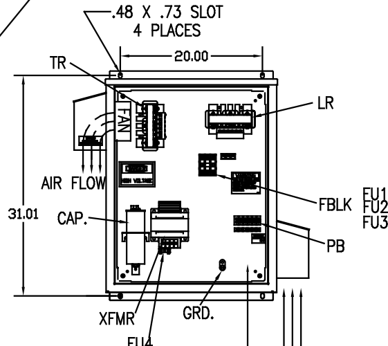
FRONT VIEW WITHOUT DOOR
